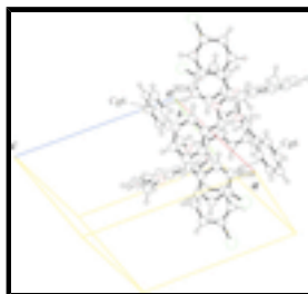
Fig. 3. A dimeric pair of the title molecules. The intermolecular \text{C—H}\cdots\pi interactions are observed along c axis (double dashed lines) [symmetry code: (ii) -x + 1, -y, -z ].
